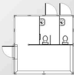
REF. XML-20/C2aa 4470 x 4470 mm. Sup. Cons. 19,99 m 2 Sup. Util 18,67 m 2
