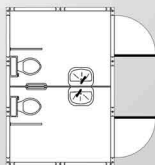
REF. AMP-2a 2360 x 3460 mm. Sup. Cons. 8,20 m 2 Sup. Útil 7,30 m 2
