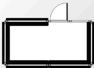
REF. XMR-4.5 2360 x 4560 mm. Sup. Cons. 10,77 m 2 Sup. Útil 9,69 m 2
